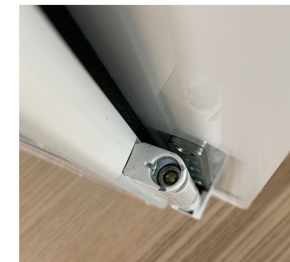
Adjustment screw on top: up and down
